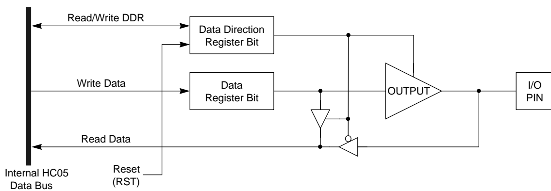
Figure 7-1. Port I/O Circuitry
