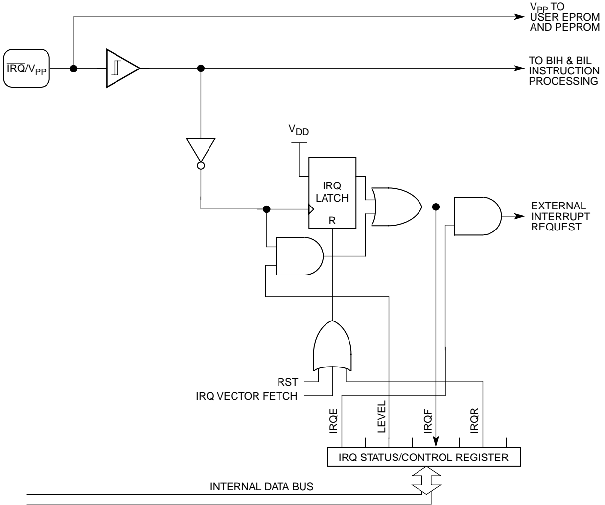
Figure 4-3. External Interrupt Logic
